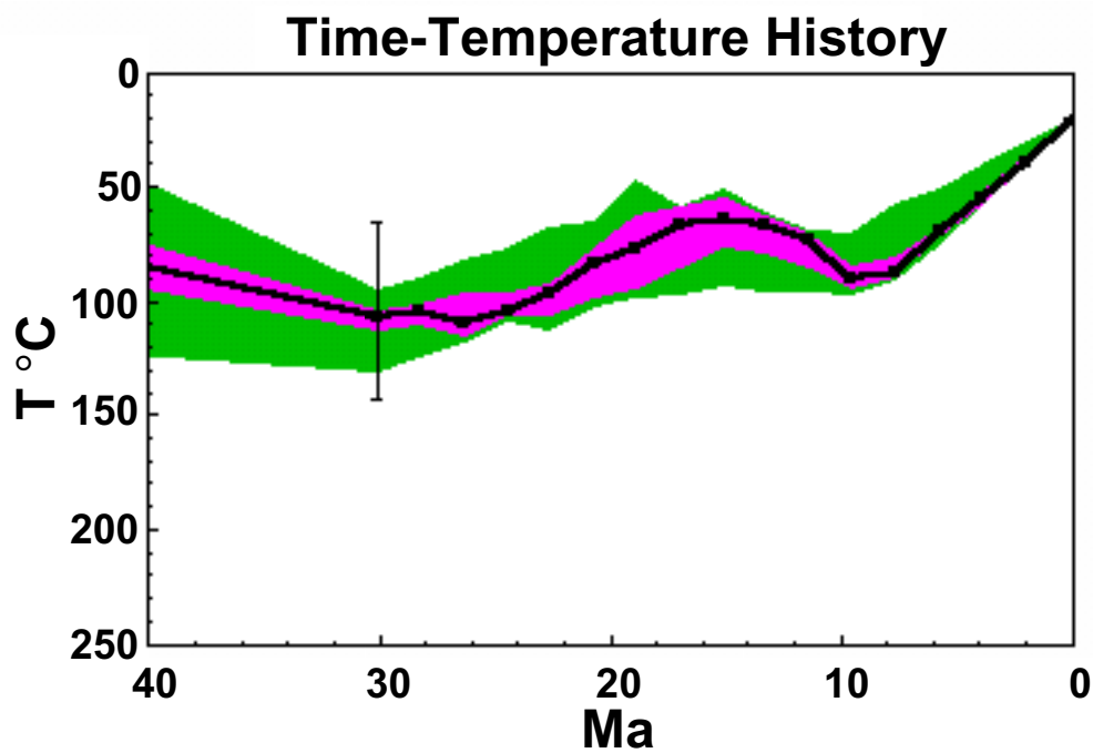
Figure 7. First attempt at inverse model of time-temperature history for sample 171-1. Thick line marks the single best-fitting t-T path found.
