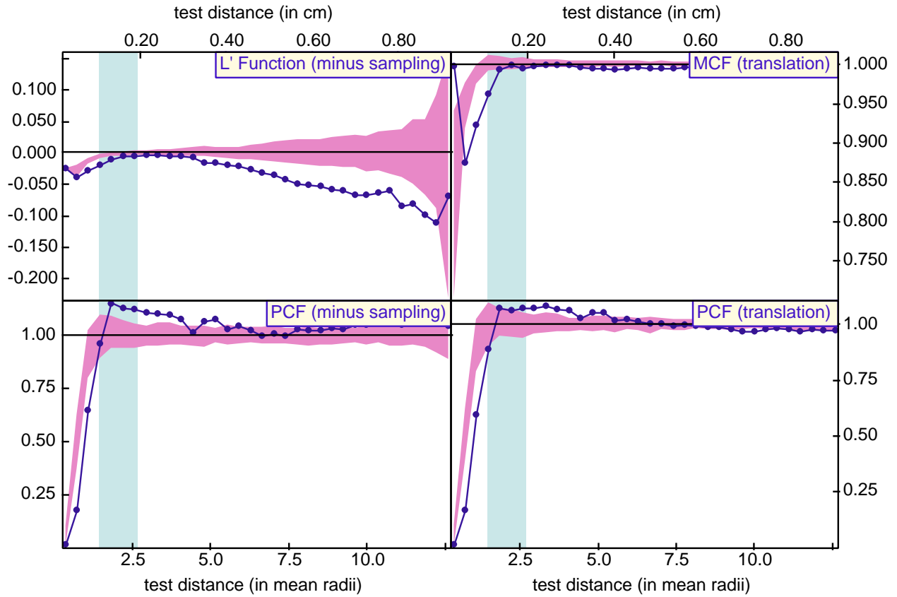
Figure 15. Correlation function data for sample PM2. The data show ordering of crystal centers and suppression of growth, in agreement with the single-valued statistics.
