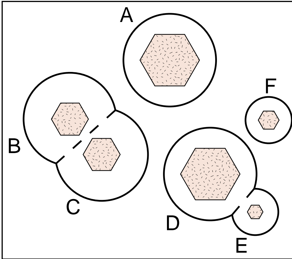
Figure 2. Schematic 2-D illustration of diffusion-controlled retardation of growth in the vicinity of a growing porphyroblast, after Carlson (1991). Competition for nutrients among closely-spaced porphyroblasts reduces the growth rates for crystals in close proximity to each other (B and C) relative to that for an isolated crystal (A) that nucleated at the same time. A crystal (E) that nucleates near the edge of the diffusionally-depleted zone of a pre-existing crystal (D) will initially have minor effects on the growth rate of the pre-existing crystal, but will itself grow more slowly than an isolated crystal that nucleated at the same time (F). Surfaces of impingement between adjacent depleted zones are the boundaries of diffusional domains; their approximate locations are marked by broken lines.
