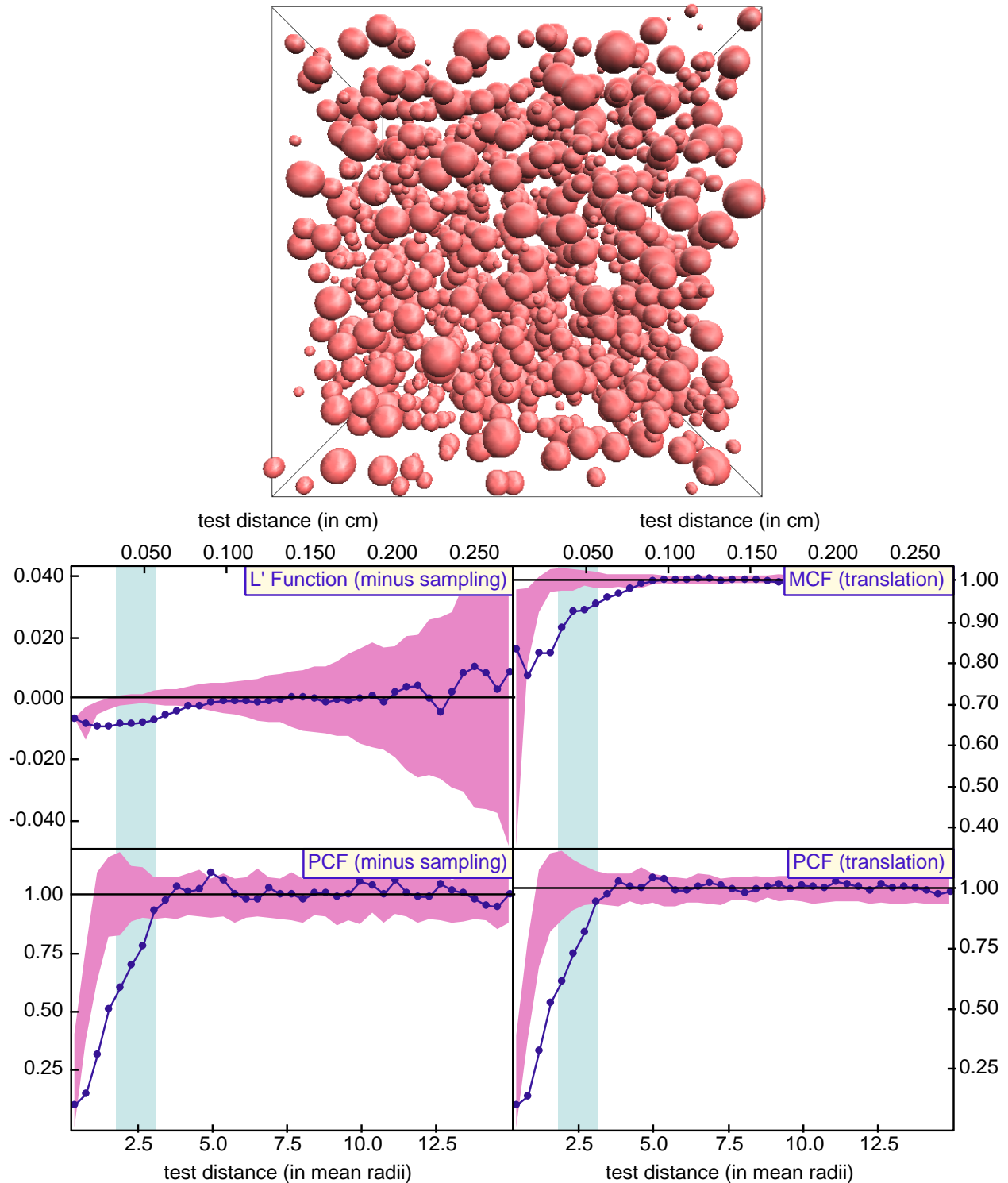
Figure 12. (a) Rendering of simulation DC-1, a thermally accelerated diffusion-controlled nucleation and growth simulation of 2971 crystals. (b) Correlation functions measured on this simulation. Data fall below the 2- \sigma envelope at scales up to the mean nearest-neighbor distance, as expected, and the MCF shows a correlation between separation and size, indicating growth suppression at small separations.
