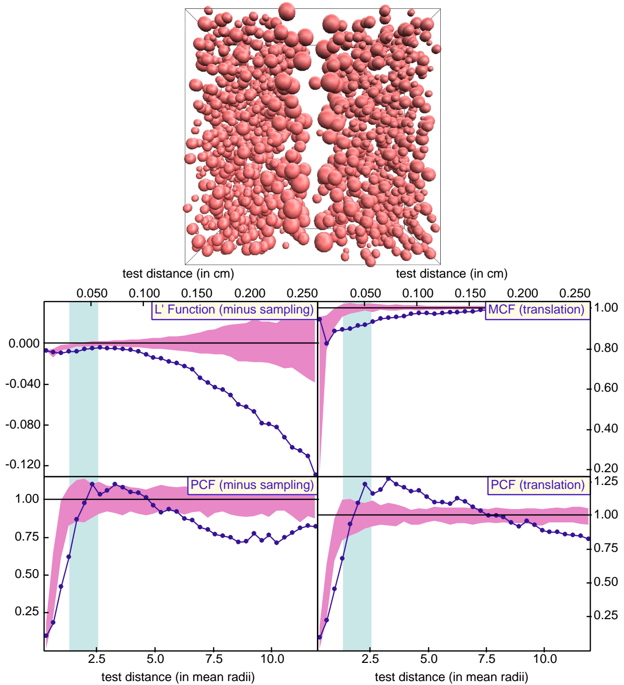
Figure 13. (a) Rendering of sub-volume of layered simulation DC-L4, in which layering is induced by a sinusoidal nucleation probability in one dimension imposed on a simulation of thermally accelerated diffusion-controlled nucleation and growth. (b) Correlation functions measured on this layered array of 1185 crystals. Envelope simulations incorporate nucleation probability distributions identical to DC-L4. Data fall below the 2\text{-}\sigma envelope at small scales, show clustering at larger scales, and then ordering at the scale of the layering, as expected. The MCF data are suspect because the simulation algorithm leads to large crystals bordering the sparse regions.
