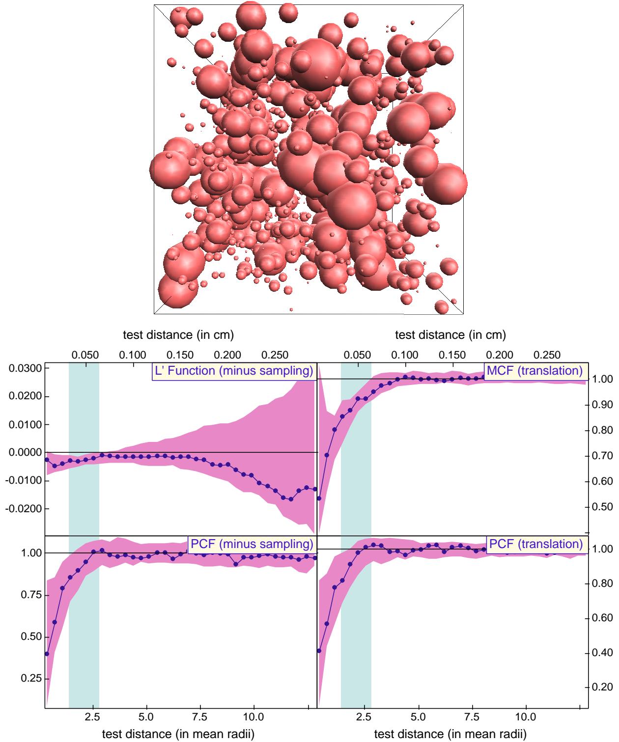
Figure 9. (a) Rendering of sub-volume of simulation IC-2, a thermally accelerated interface-controlled nucleation and growth simulation of 1739 crystals. (b) Correlation functions measured on this simulation; data fall within the 2- \sigma envelope, as expected.
