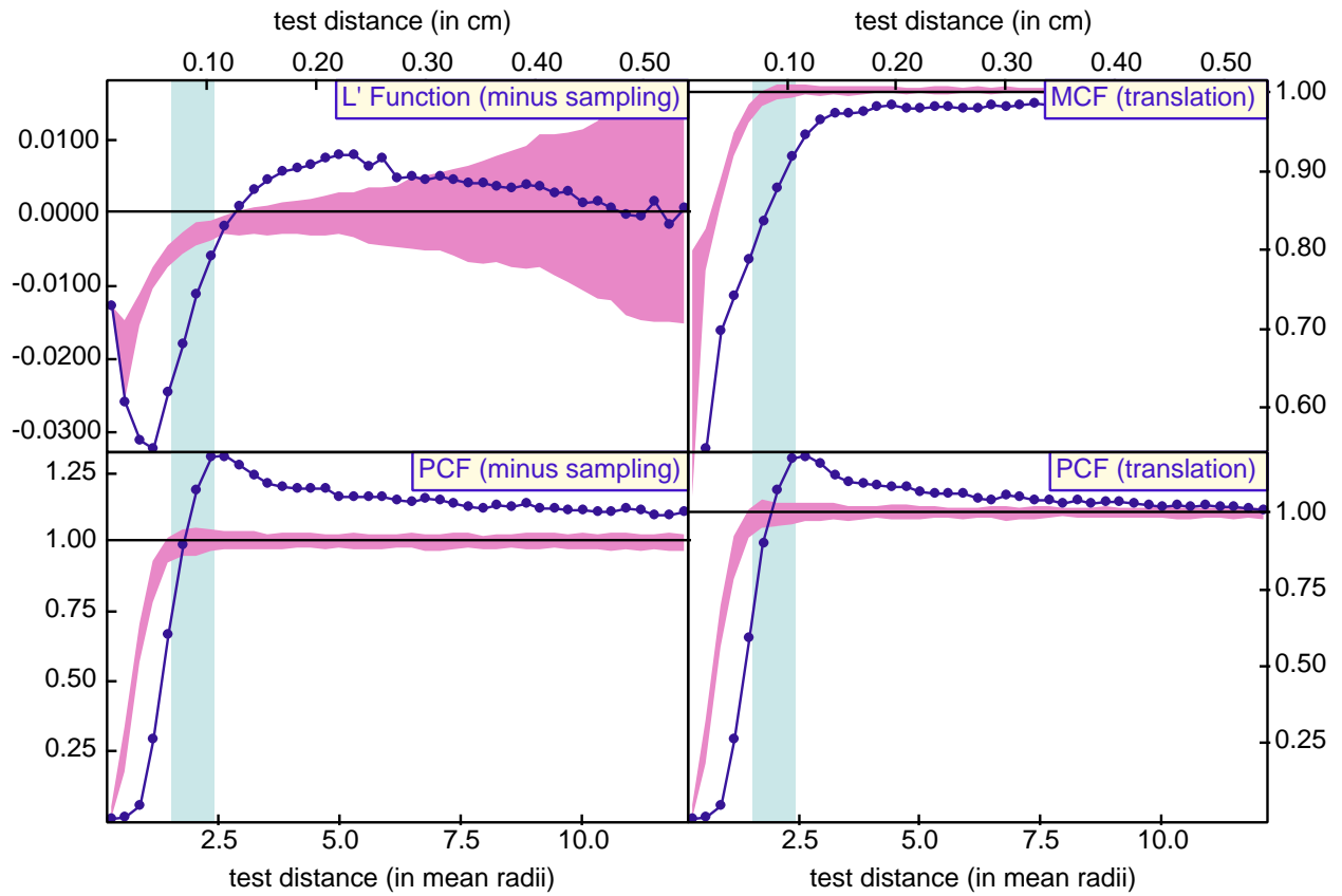
Figure 19. Correlation function data for sample WR3. The data show ordering of crystal centers and suppression of growth, in agreement with the single-valued statistics.
