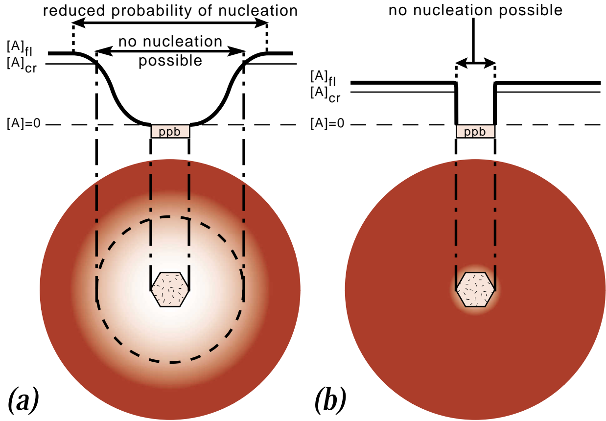
Figure 1. Schematic 2-D illustration of diffusion-controlled suppression of nucleation in the vicinity of a growing porphyroblast ("ppb"), after Carlson (1989). (a) If diffusion is sluggish relative to interfacial reaction, then near a growing porphyroblast slow diffusion produces gradients in the chemical affinity for the crystallization reaction in the intergranular fluid [A]_{fl} . This results in zones of zero probability of nucleation where the intergranular chemical affinity is less than the critical value required to overcome the activation energy for nucleation [A]_{cr} . These zones are surrounded by zones of reduced probability of nucleation where the chemical affinity is less than the value in regions unaffected by diffusion, but greater than the critical value. (b) If diffusion is rapid, then the only significant effect is the prevention of nucleation within the volume of a pre-existing porphyroblast.
