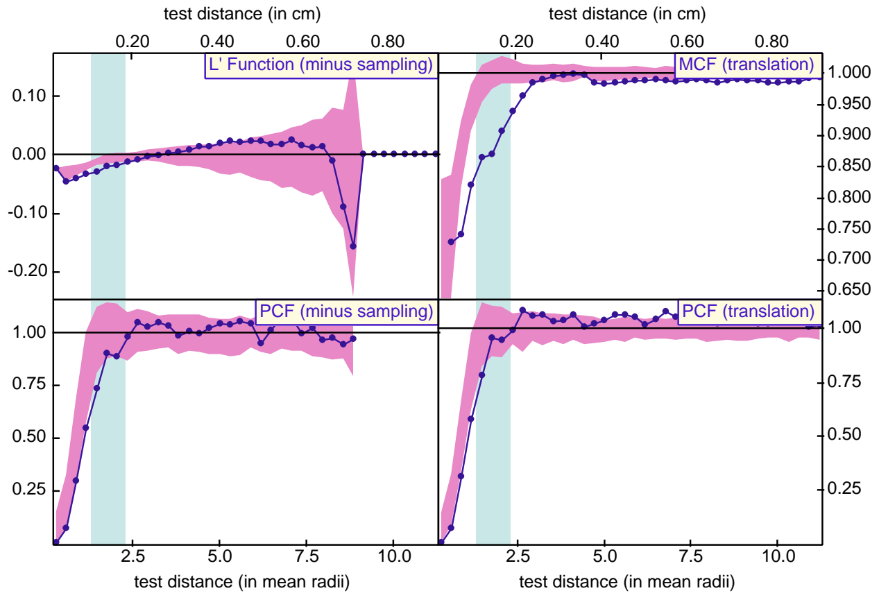
Figure 17. Correlation function data for sample WR1. The data show ordering of crystal centers and suppression of growth, in agreement with the single-valued statistics.
