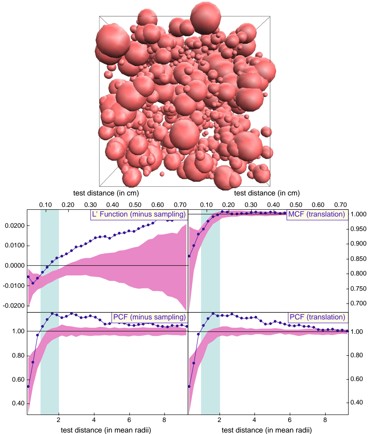
Figure 11. (a) Rendering of simulation IC-WR1, a thermally accelerated interface-controlled nucleation and growth simulation of 5096 crystals with clustering induced by sinusoidal nucleation probability in each dimension. (b) Correlation functions measured on this simulation. The data fall above the 2- \sigma envelope at all scales but the smallest, reflecting the clustering of the simulation; the MCF data show no growth suppression, however.
