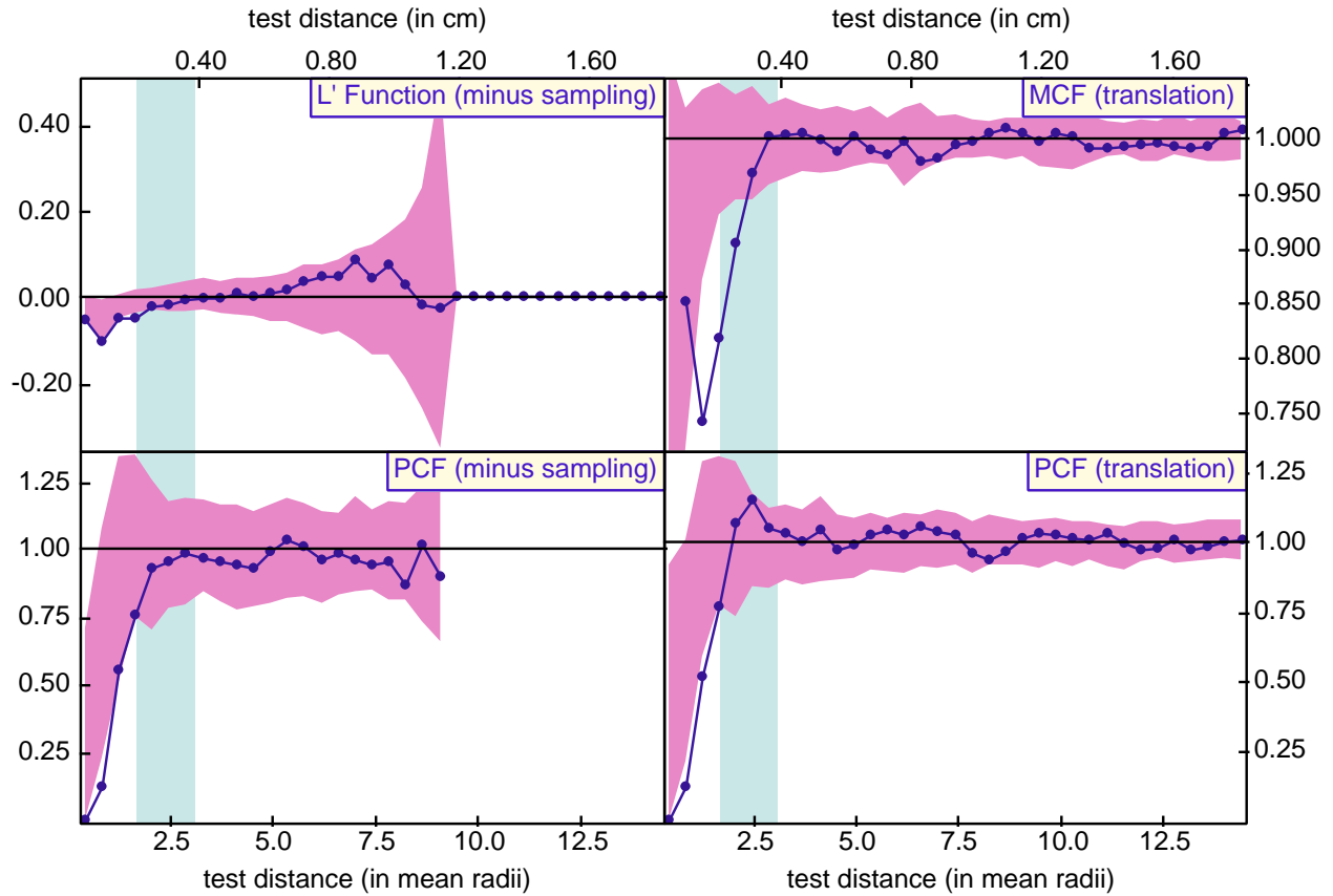
Figure 16. Correlation function data for sample MD. The data show slight negative excursions below the null-hypothesis region for the L' function and PCF, indicating barely significant ordering of crystal centers, and a strong excursion below the envelope for the MCF, indicating growth suppression for closely spaced crystals.
