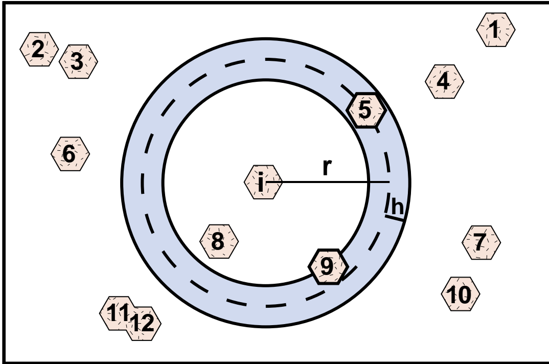
Figure 4. Schematic 2-D illustration of measurement regions for the Pair Correlation and Mark Correlation Functions. For each crystal i in the sample, each other crystal j whose center lies within a spherical annulus (shaded ring) of thickness 2h and radius r centered at crystal i is counted. In this illustration, the crystals outlined in bold ( j=5 , and j=9 ) will be counted in the summand for crystal i ; the others will not.
