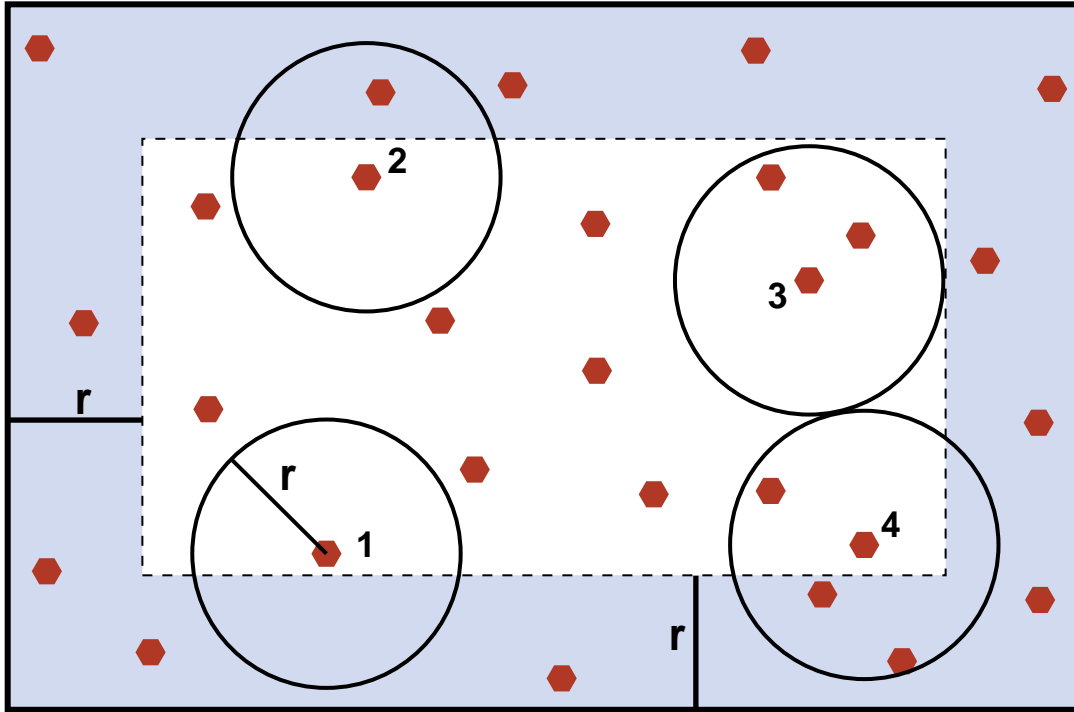
Figure 7. Schematic 2-D illustration of "minus-sampling" edge-correction method. A guard region (wide shaded border region) of the same thickness as the test distance, r , is placed inside the sample boundary. The iteration over crystals i (placement of measurement region) is prohibited from this region, although they may be counted as crystals j within measurement regions. This effectively prohibits the measurement regions from ever intersecting the sample boundary. Four allowable measurement regions are shown as solid circles.
