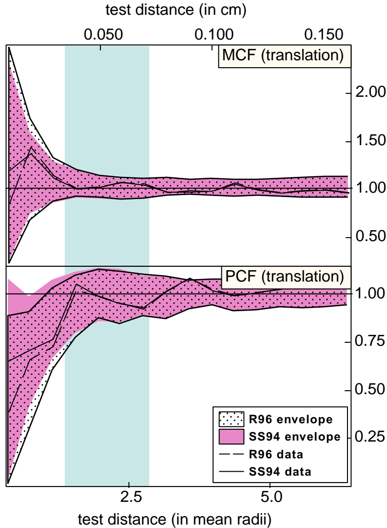
Figure 6. Comparison between the present versions of the MCF and PCF (taken from Stoyan and Stoyan, 1994, "SS94") and those proposed by Raeburn (1996), "R96", performed on the random simulation given in Figure 9. The Raeburn statistic is systematically slightly lower than the present version, particularly at small test distances, but because it is also used to measure the envelopes, compensating errors may leave the conclusion unchanged.
