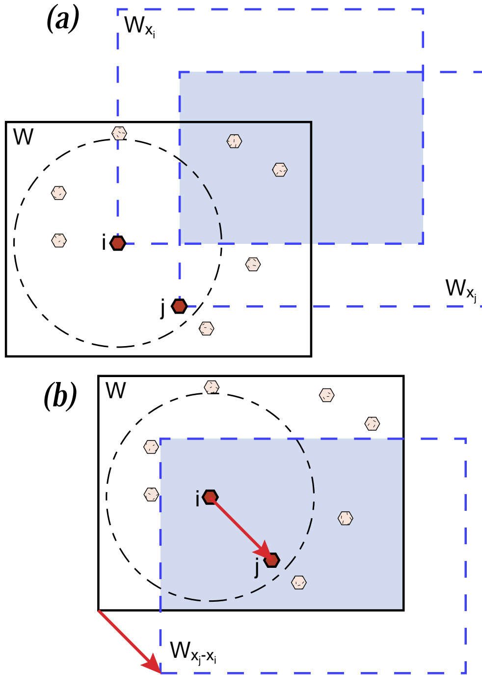
Figure 8. Schematic 2-D illustration of translation edge-correction method. For the pair of crystals in bold, i and j , the summand is divided by the volume of the shaded region. (a) As defined in Stoyan and Stoyan (1994), this region is W_{x_i} \cap W_{x_j} , the intersection of the sample region W offset to each of the crystals in the pair. (b) This volume is equivalent to W \cap W_{x_j - x_i} , the intersection of the sample region W and that region offset by the vector from the center of crystal i to the center of crystal j . The value of the summand is normalized by this intersection volume for each pair counted.
