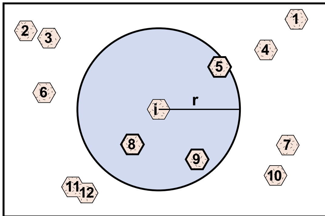
Figure 3. Schematic 2-D illustration of measurement regions for the K , L , and L' functions. For each crystal i in the sample, each other crystal j whose center lies within a sphere of radius r (shaded circle) centered at crystal i is counted. In this illustration, the crystals outlined in bold ( j=5 , j=8 , and j=9 ) will be counted in the summand for crystal i ; the others will not.
