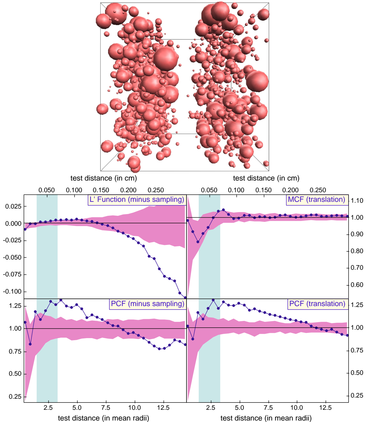
Figure 10. (a) Rendering of sub-volume of layered simulation IC-L2, in which layering is induced by a sinusoidal nucleation probability in one dimension imposed on a simulation of thermally accelerated interface-controlled nucleation and growth. (b) Results of correlation functions measured on this layered array of 1172 crystals. Data show clustering up to about 10 mean radii ( \sim 0.2 cm), and fall below the 2\text{-}\sigma envelope at greater length scales, reflecting the relative sparsity of crystals beyond the scale of layering; the MCF data show no growth suppression, as expected from input parameters of simulation IC-L2.
