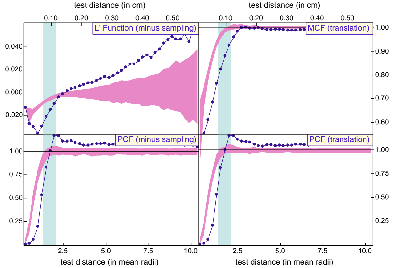
Figure 18. Correlation function data for sample WR2. The data show ordering of crystal centers and suppression of growth, in agreement with the single-valued statistics.
