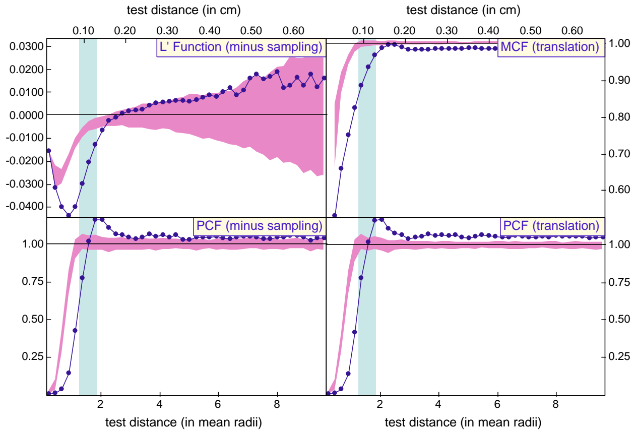
Figure 14. Correlation function data for sample PM1. The data show the result expected from the single-valued statistics: both ordering and growth suppression up to about the mean nearest-neighbor distance.
