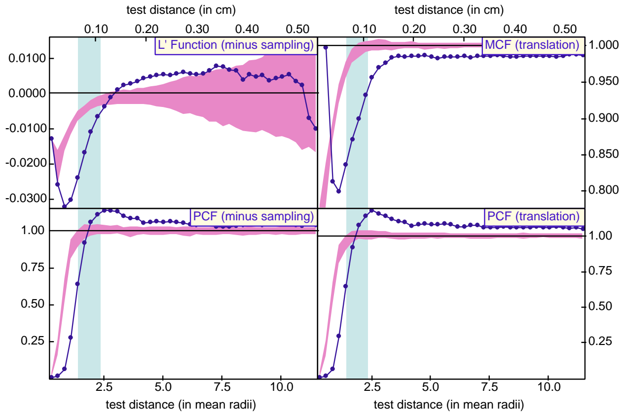
Figure 20. Correlation function data for sample WR4. The data show ordering of crystal centers and suppression of growth, in agreement with the single-valued statistics.
